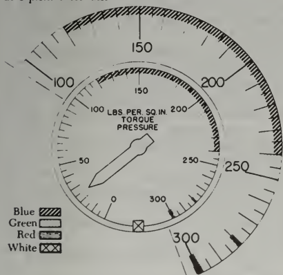
FIGURE 10-30. Torquemeter.
